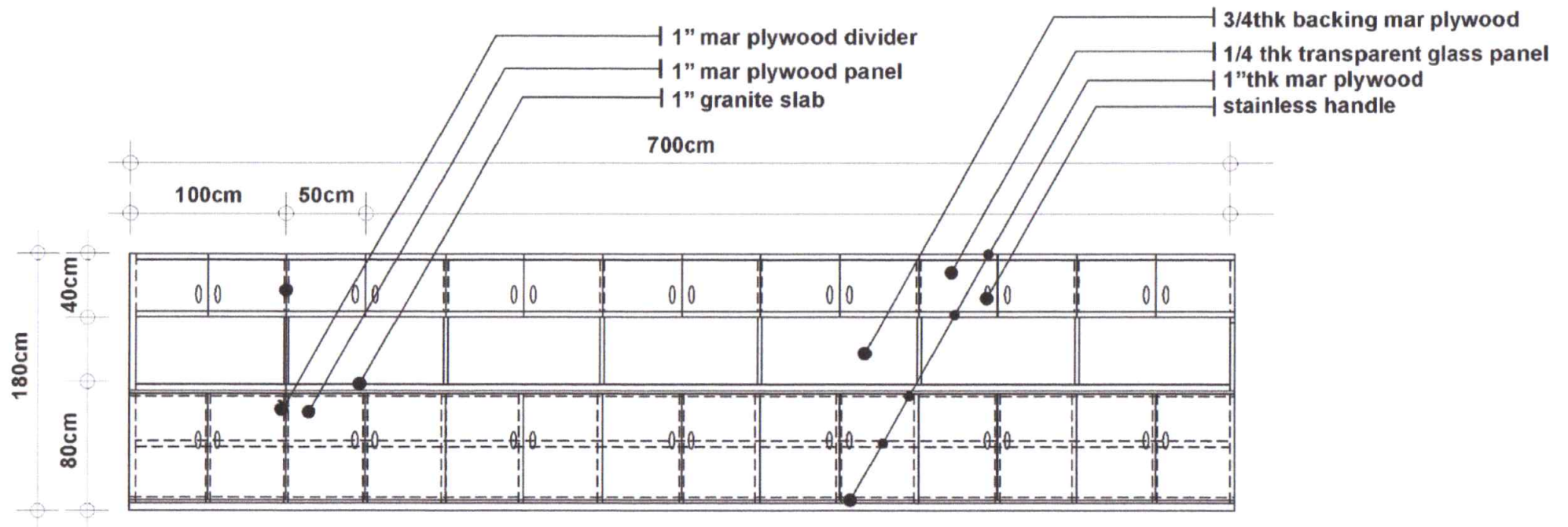
FRONT VIEW
